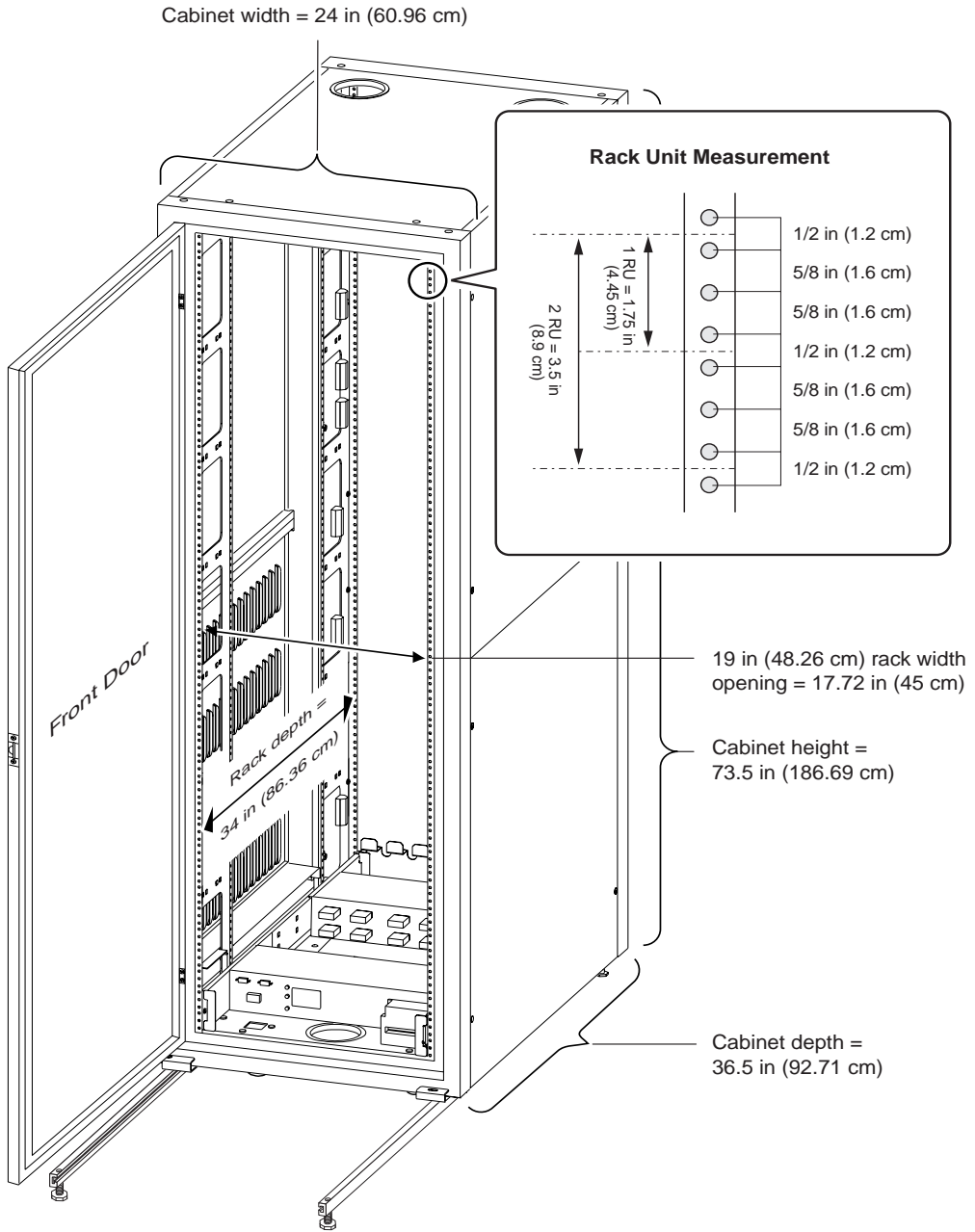
FIGURE 2-2 EIA 310-Compliant Cabinet and Rack
